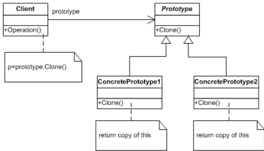
Prototype
