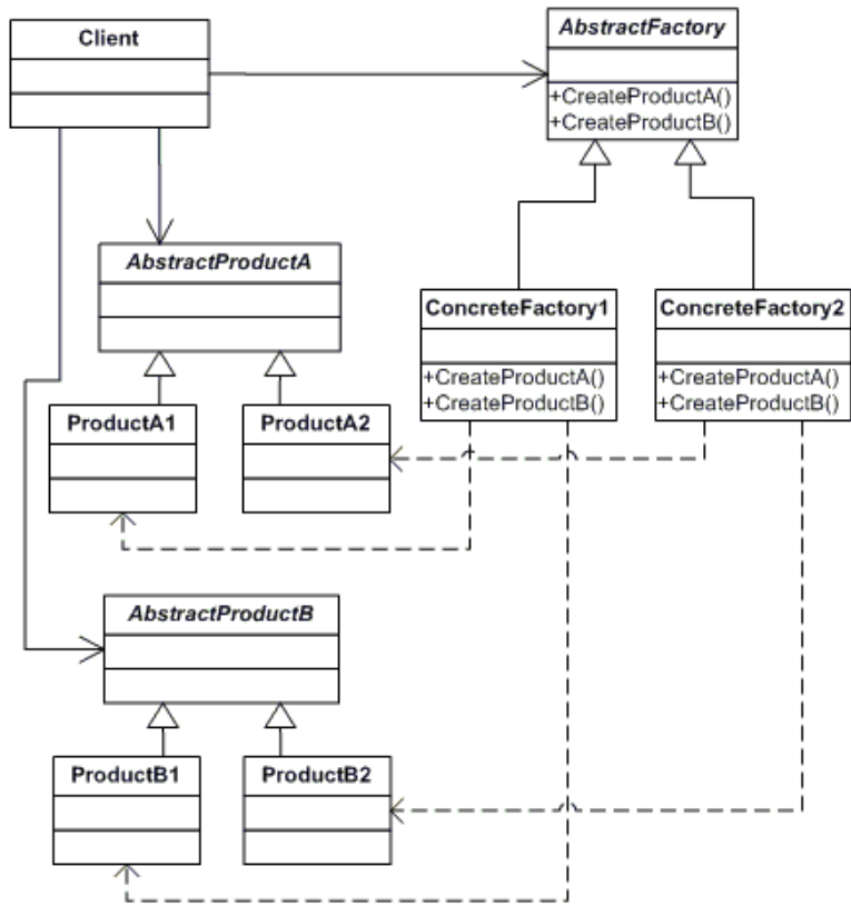
Abstract Factory
