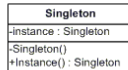
Singleton
