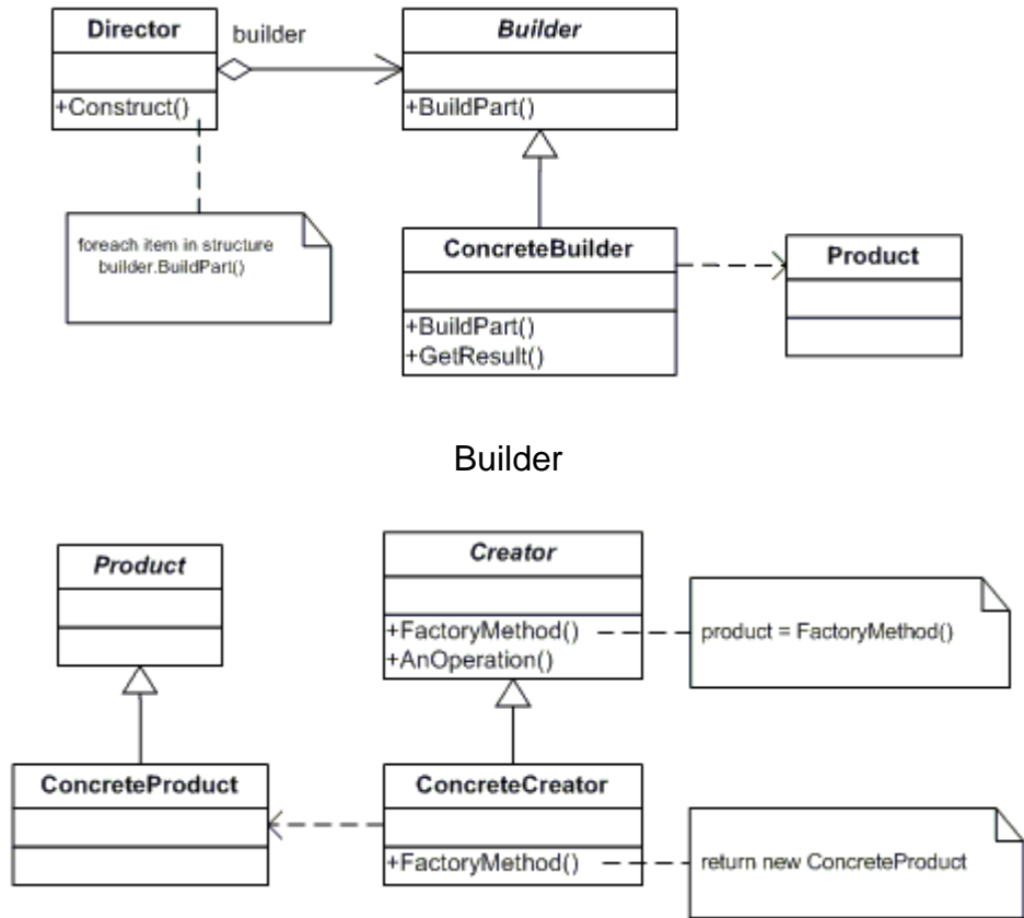
Factory Method
